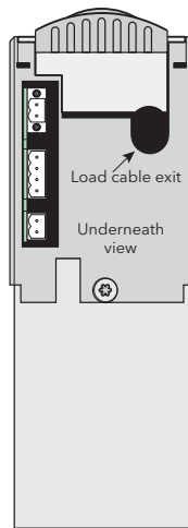
External Feedback Connector Pinout and Polarising Details
