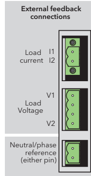
External Feedback Connector Pinout and Polarising Details
